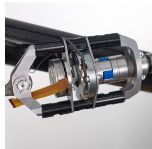
Fig. 5. Built-in actuation with cover removed showing the motor, brake and coupling (from left to right)
