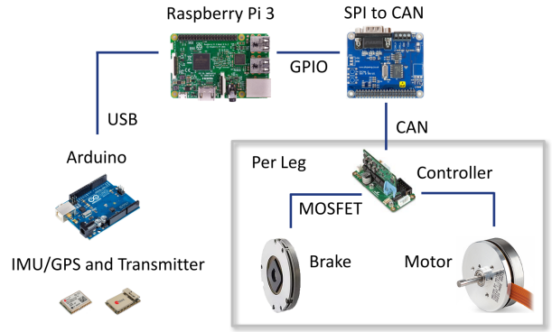
Fig. 9. Overview of all electronic hardware components
